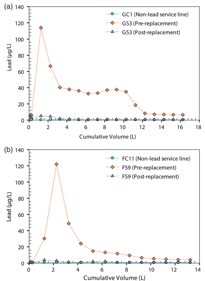
FIGURE 5 Examples of sequential sampling of lead profiles in homes of two cities (a and b). Profiles were obtained in homes before and after lead service line replacement, and in homes that never had a lead service line. The illustrative trends are meant to indicate lead service line presence or absence. The exact lead concentrations are specific to the sampled homes. They should not be generalized to reflect other homes, which may have different plumbing and/or water chemistry characteristics
