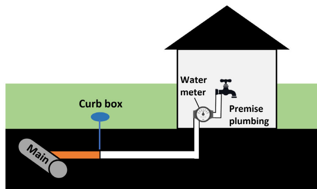
FIGURE 3 Typical example of privately owned and publically owned lead service lines based on curb stop division (modified diagram from Deshommes et al., 2016). Water meter may be located outside or inside the building. For some materials, a gooseneck may be present, connecting the water main and the publicly owned service line
