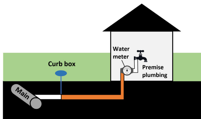
FIGURE 3 Typical example of privately owned and publically owned lead service lines based on curb stop division (modified diagram from Deshommes et al., 2016). Water meter may be located outside or inside the building. For some materials, a gooseneck may be present, connecting the water main and the publicly owned service line
